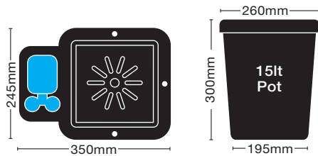
Complete 1Pot System with 47lt tank (includes all pipework and fittings)
