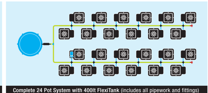
Complete 24 Pot System with 400lt FlexiTank (includes all pipework and fittings)
