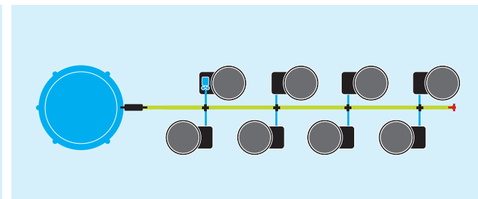
Complete SmartPot 8 System with 100lt FlexiTank (includes all pipework and fittings)
