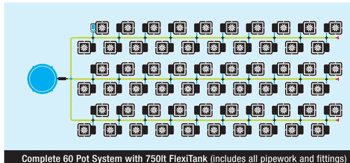
Complete 60 Pot System with 750lt FlexiTank (includes all pipework and fittings)
