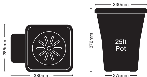
Complete 1Pot System with 47lt tank (includes all pipework and fittings)
