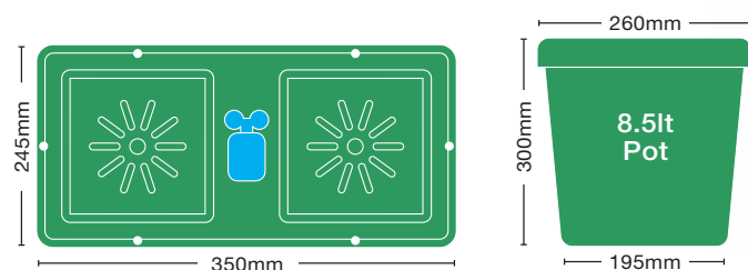
Complete easy2grow System with 47lt tank (includes all pipework and fittings)
