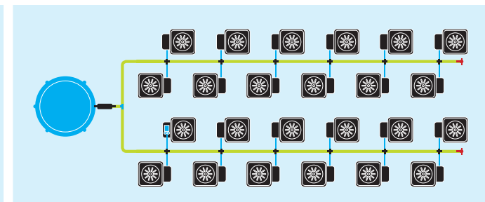
Complete 24Pot XL System with 400lt FlexiTank (includes all pipework and fittings)
