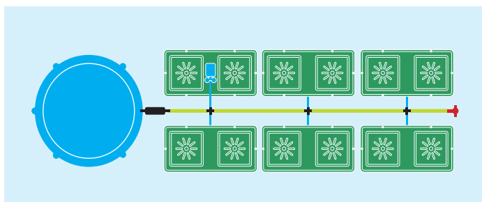
Complete easy2grow 12 System with 100lt FlexiTank (includes all pipework and fittings)
