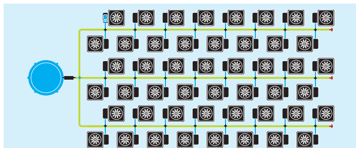
Complete 48Pot XL System with 400lt FlexiTank (includes all pipework and fittings)
