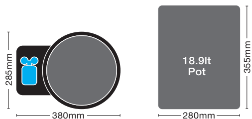
Complete easy2grow System with 47 litre tank (includes all pipework and fittings)
